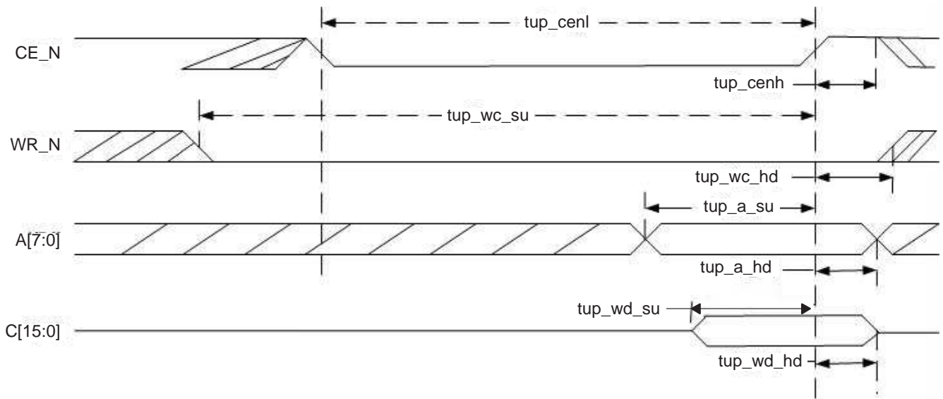
Figure 14. Write Cycle \overline{RD} Held Low
