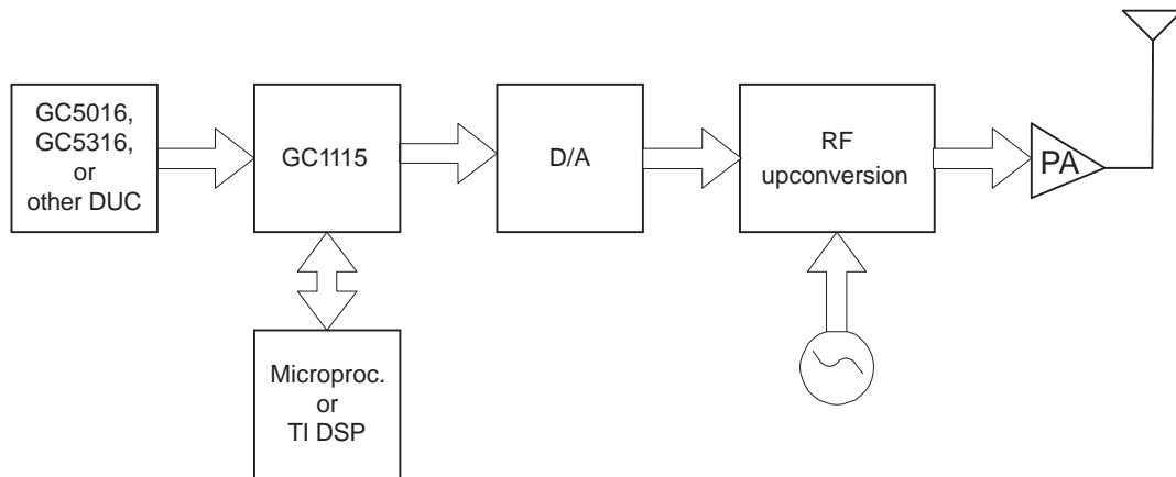
Figure 1. Wireless System Using the GC1115
